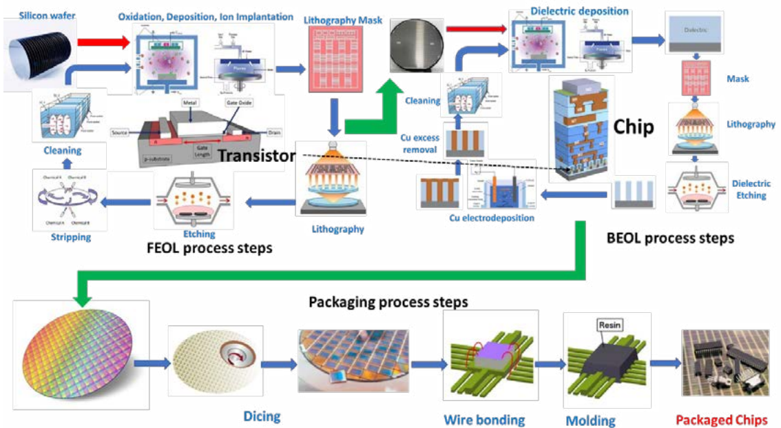
Figure 1: Schematic overall process for manufacturing chips for logic devices
